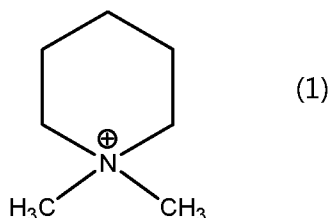
N,N -dimethylpiperidinium cation
