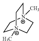
N,N'-dimethyl-1,4-diazabicyclo[2.2.2]octane dication
