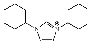
1,3-dicyclohexylimidazolium cation
